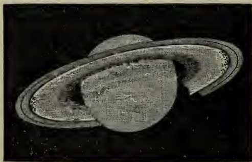
Fig. 2.—Saturn, as observed by Trouvelot with the 26-inch Washington Refractor.
