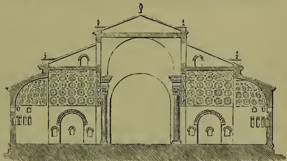
Fig. 3.—Transverse Section of Basilica of Maxentius.
