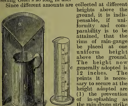
Symons' Rain-gauge.
